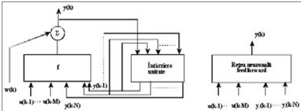
Fig. 5. The used model
