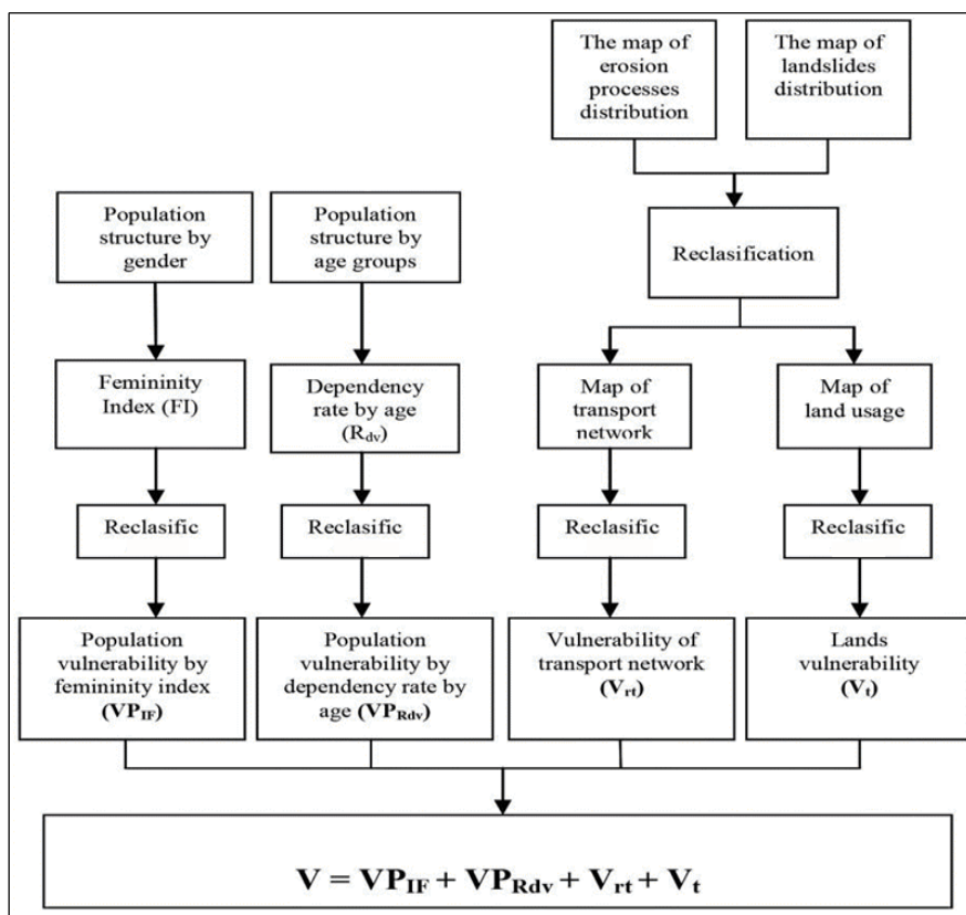
Fig. 7. Scheme of analysis of population vulnerability to current geomorphological processes.
