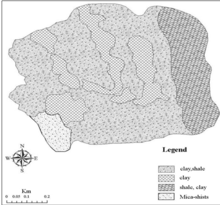
Fig. 2. Geological map of study area
