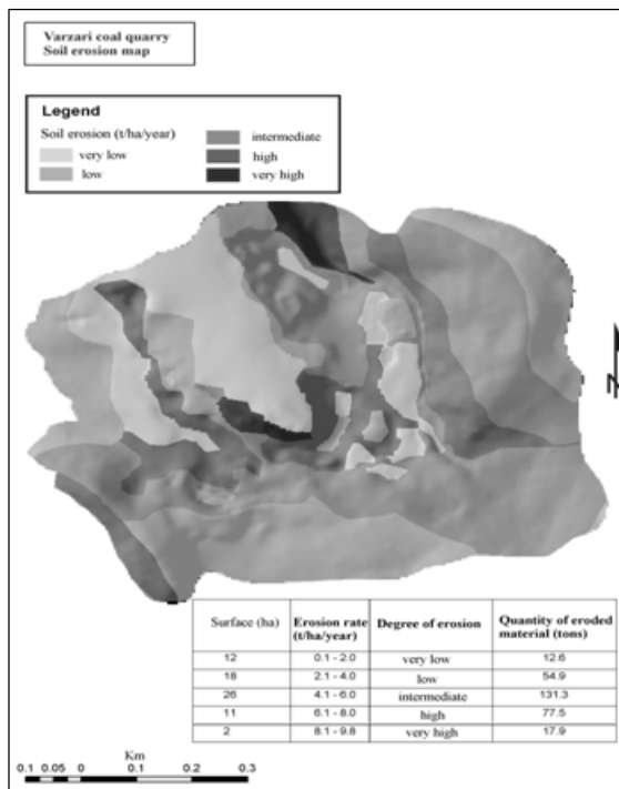
Fig. 6. Soil erosion map of coal quarry
