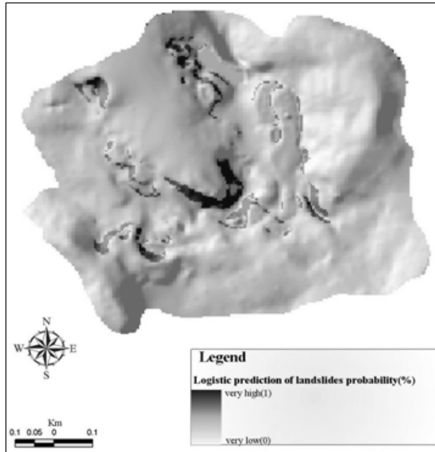
Fig. 4. Landslide prediction map of coal quarry
