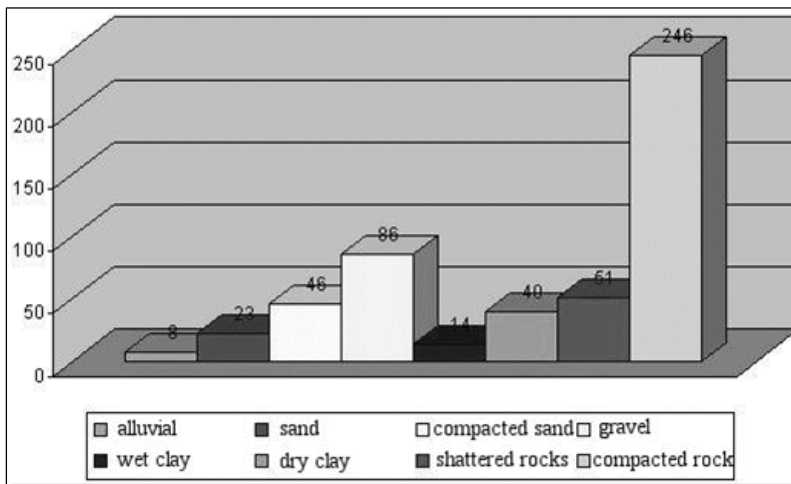
Fig. 3. Support capacity of different types of materials (Beer, 1990)
